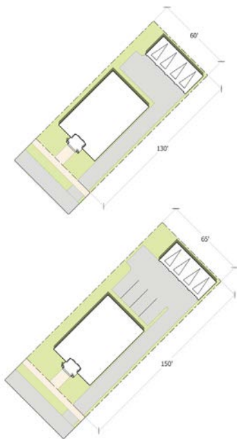
Figure 4.11 Parking has a significant impact on MMH and affordability. This illustration shows how much more space is required to fit a quadplex on a lot when 2 spaces are required per unit versus 1 space per unit.
